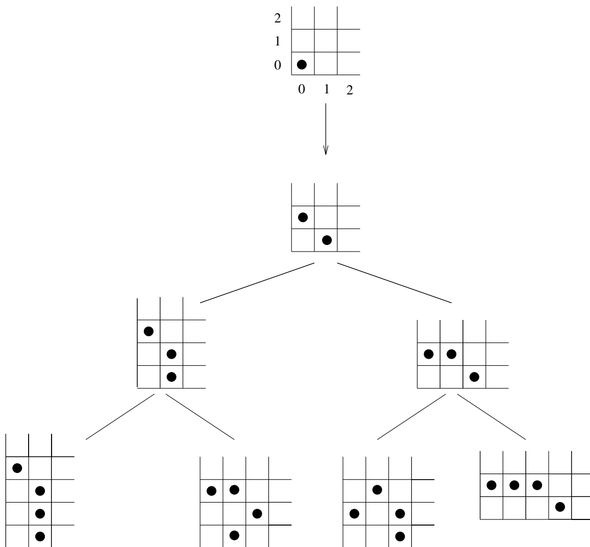
Figure 2: Reachable configurations with at most four pebbles.
