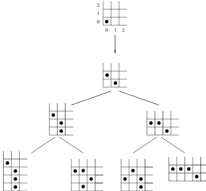
Figure 2: Reachable configurations with at most four pebbles.
