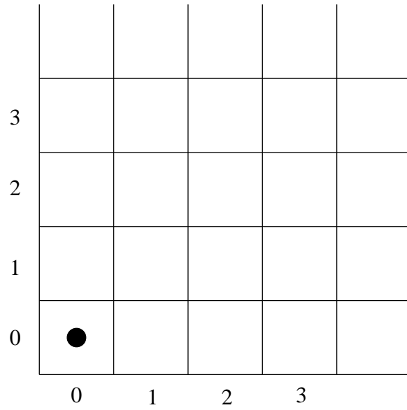
Figure 1: The starting configuration on the board B .
