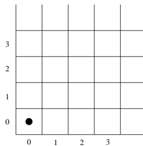
Figure 1: The starting configuration on the board B .
