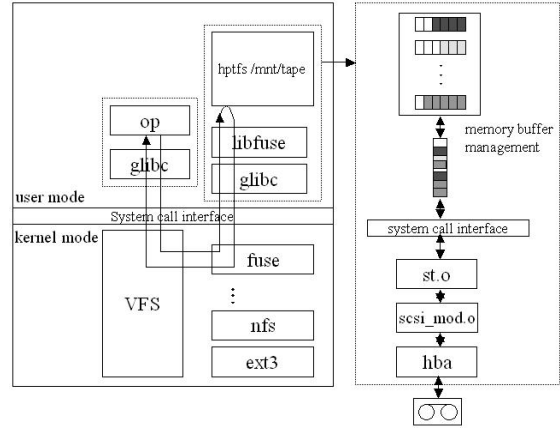
Fig. 1. Architecture of HPTFS
