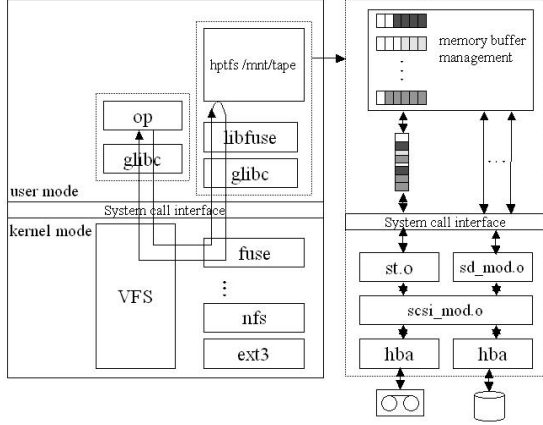
Fig. 5. Continuous Data Protection
