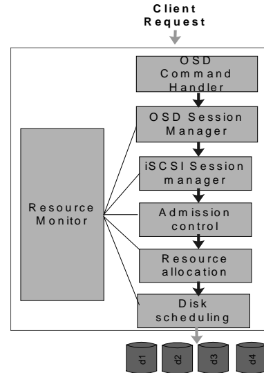
Figure 3. QoS framework in OSD
