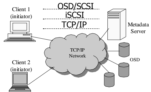
Figure. 1 OSD-based system
