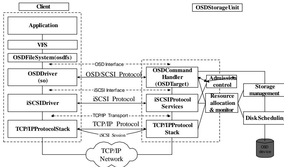
Figure 4. The software architecture
